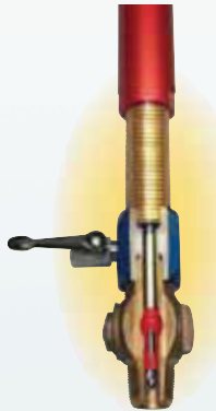
Cutaway View
